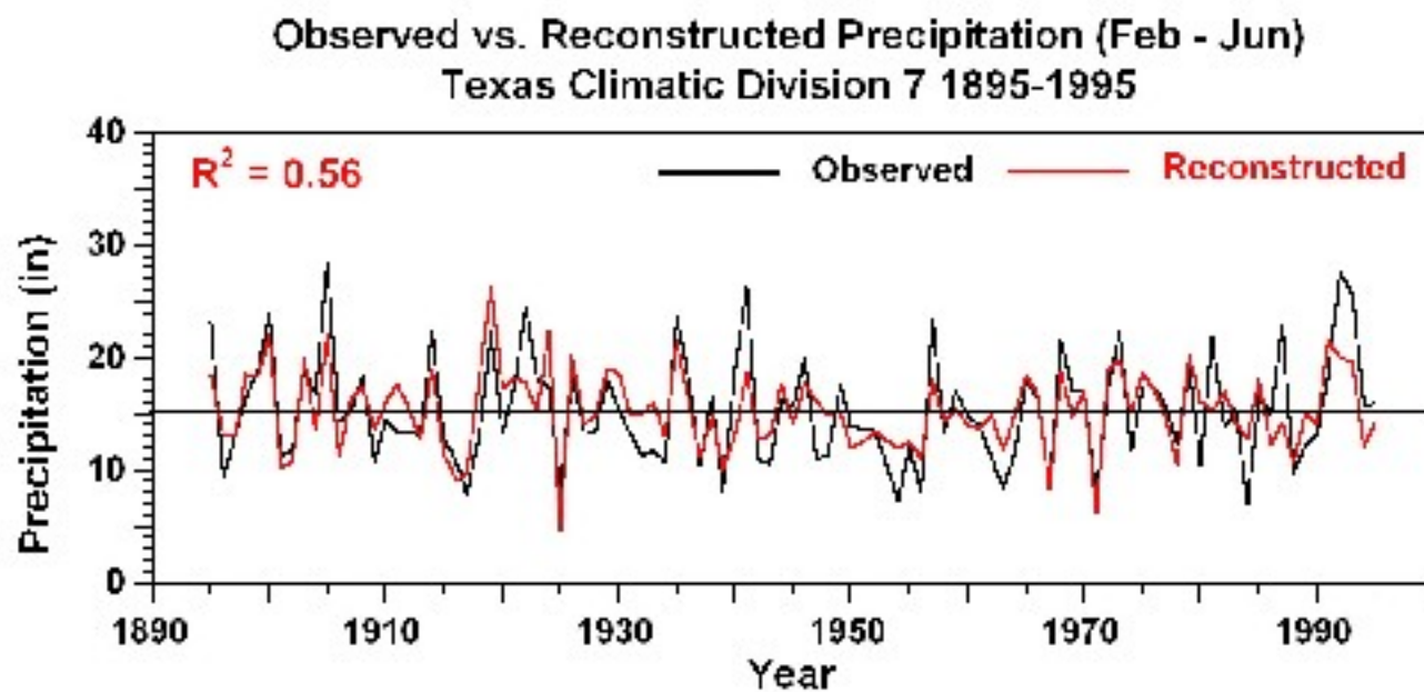
Figure 2. Calibration of Texas climate division South Central with a composite post oak chronology.
