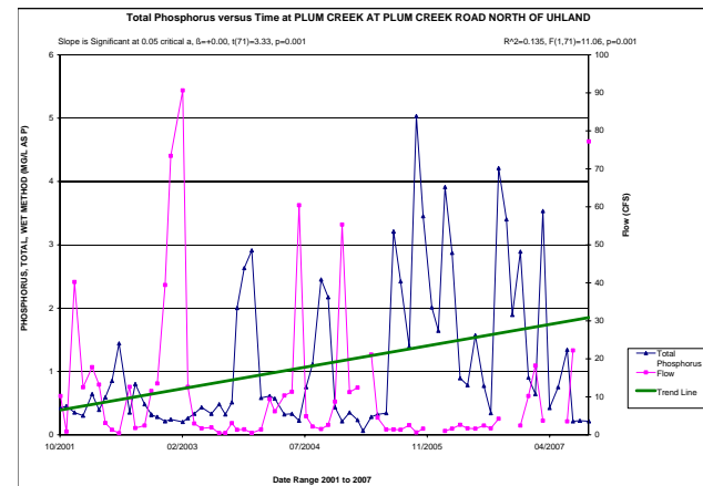
Figure 1. At the GBRA monitoring location at Plum Creek at Plum Creek Road (17406) near Uhlend, there is an inverse relationship between flow and total phosphorus.
