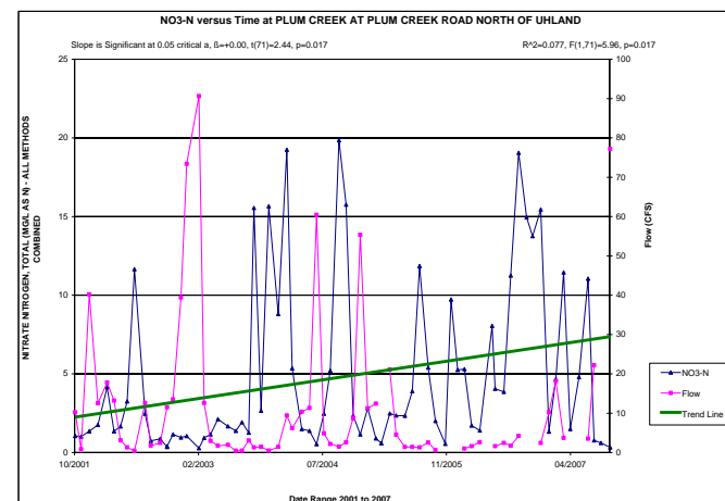
Figure 2. Concentration of nitrate nitrogen showing an increasing trend over time at the Plum Creek at Plum Creek Road (17406). Spikes attributed to periods of low flow when the stream becomes dominated by wastewater effluent.
